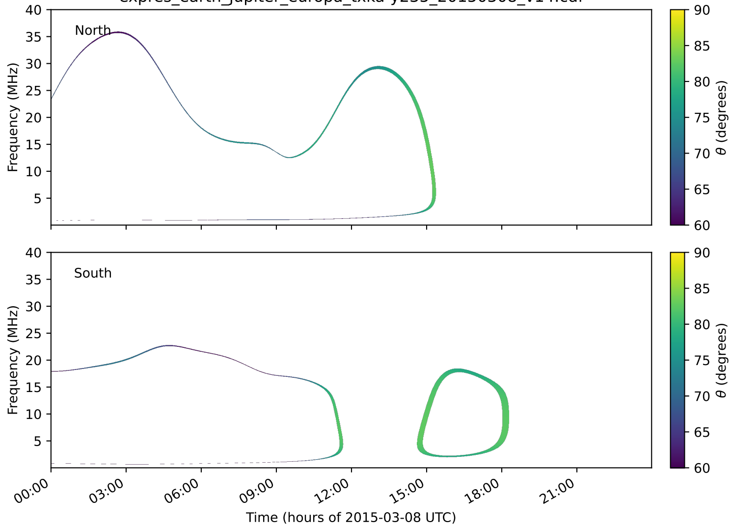
expres_earth_jupiter_europa_txka-y235_20150308_v14.cdf
