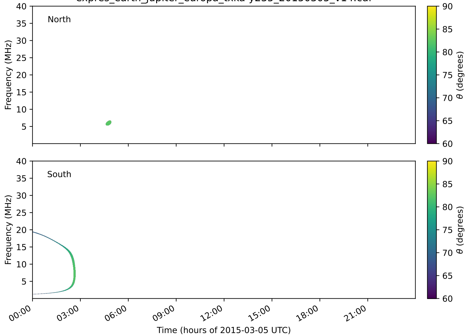
expres_earth_jupiter_europa_txka-y235_20150305_v14.cdf
