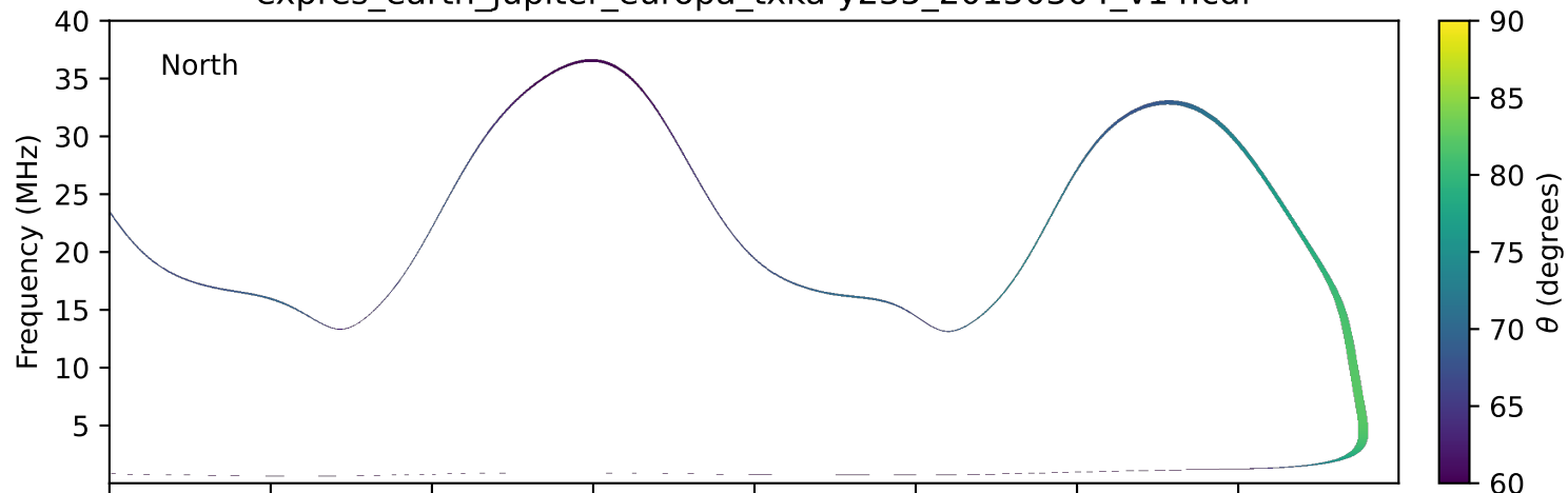
expres_earth_jupiter_europa_txka-y235_20150304_v14.cdf
