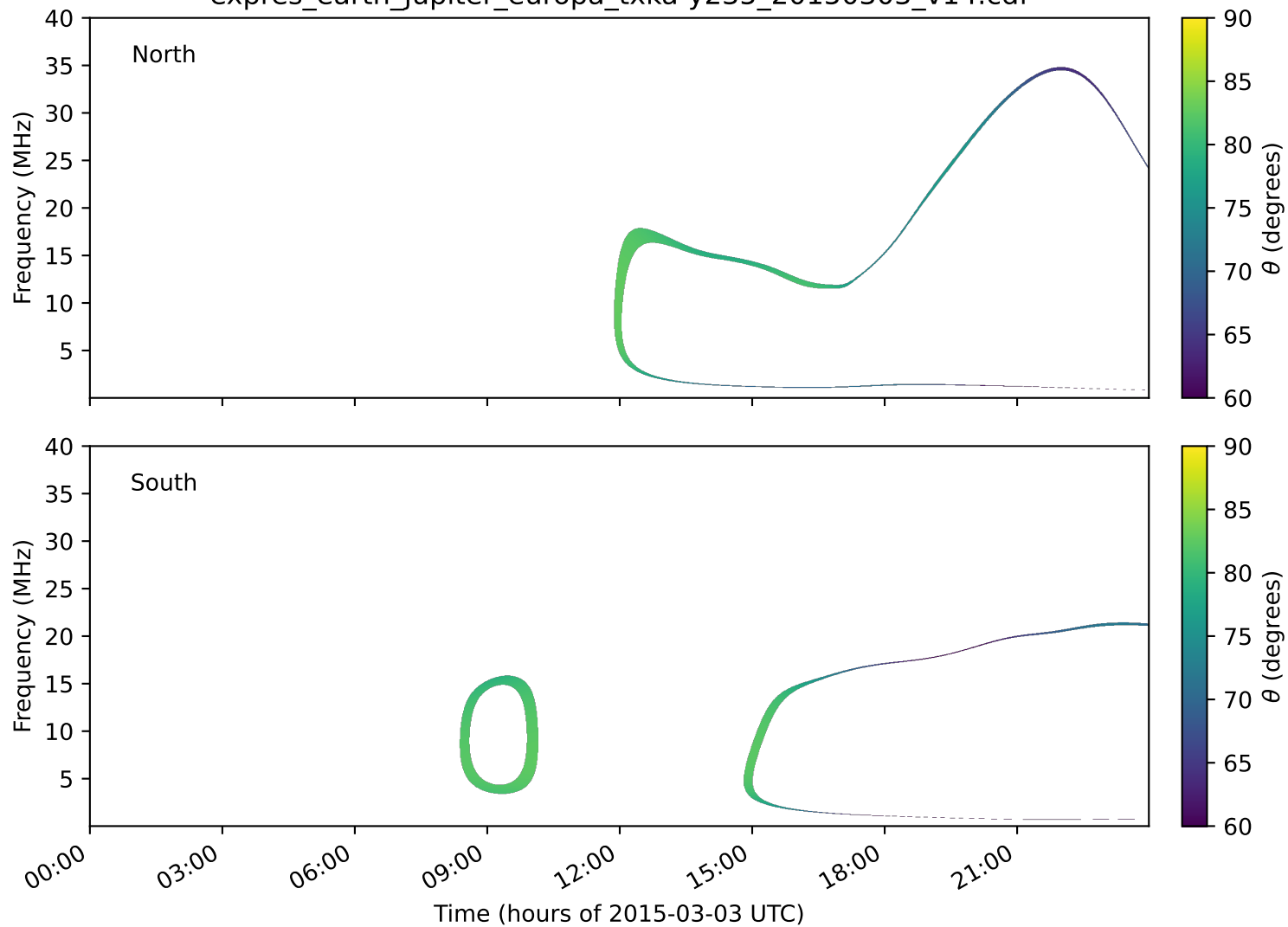
expres_earth_jupiter_europa_txka-y235_20150303_v14.cdf
