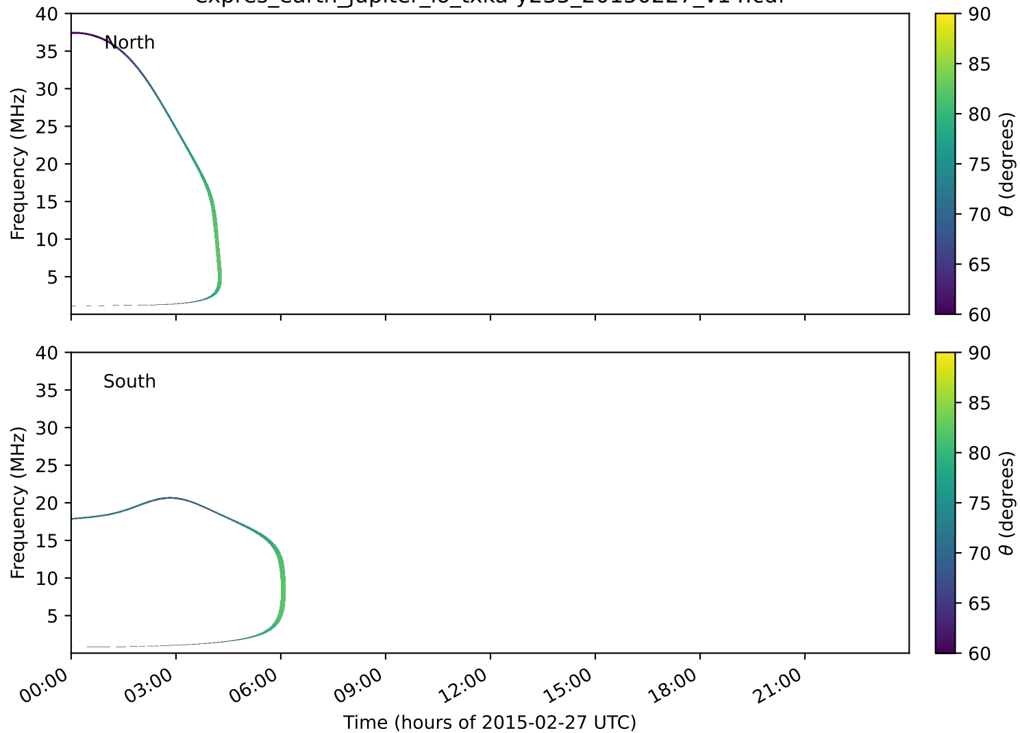
expres_earth_jupiter_io_txka-y235_20150227_v14.cdf
