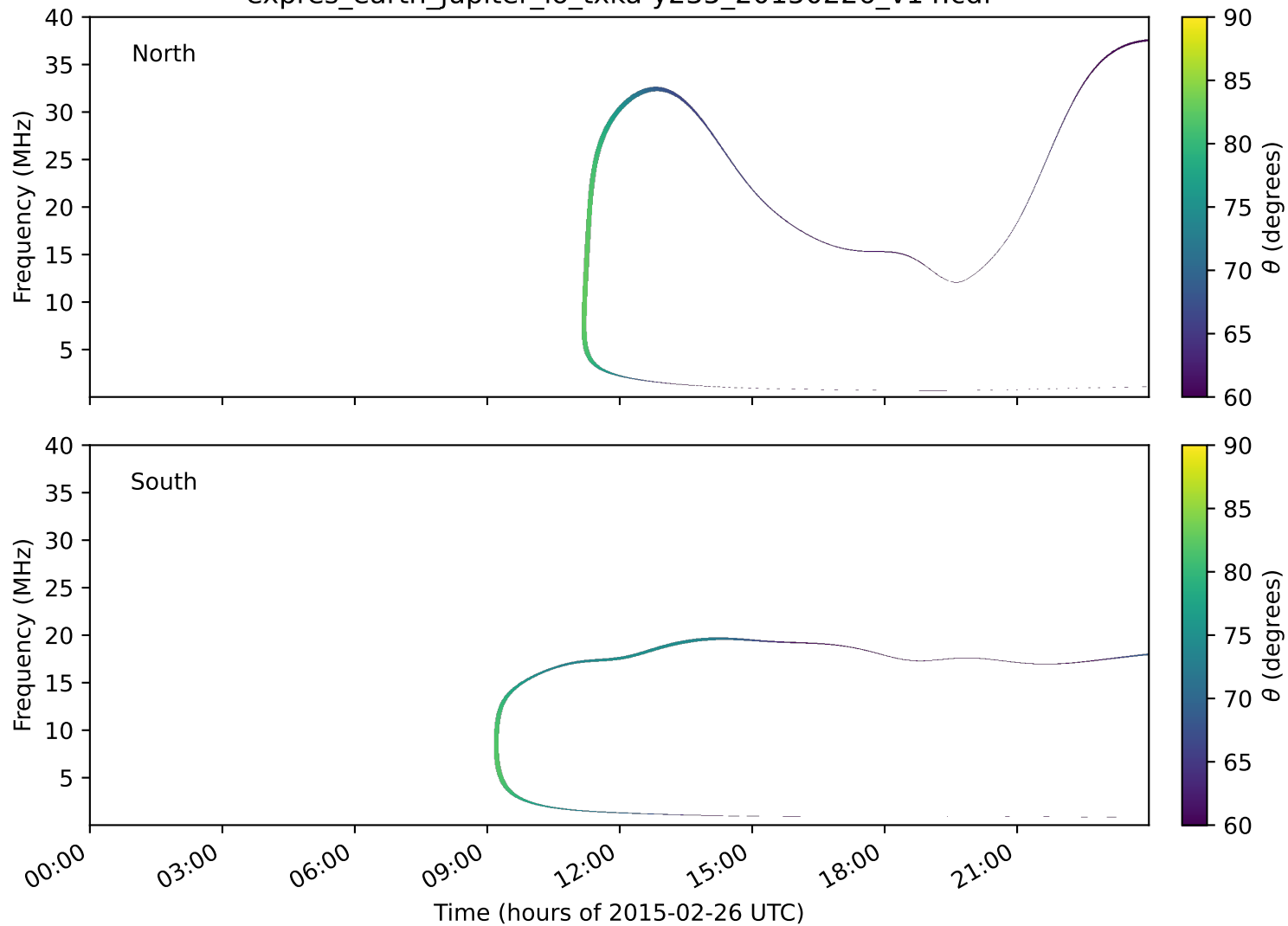
expres_earth_jupiter_io_txka-y235_20150226_v14.cdf
