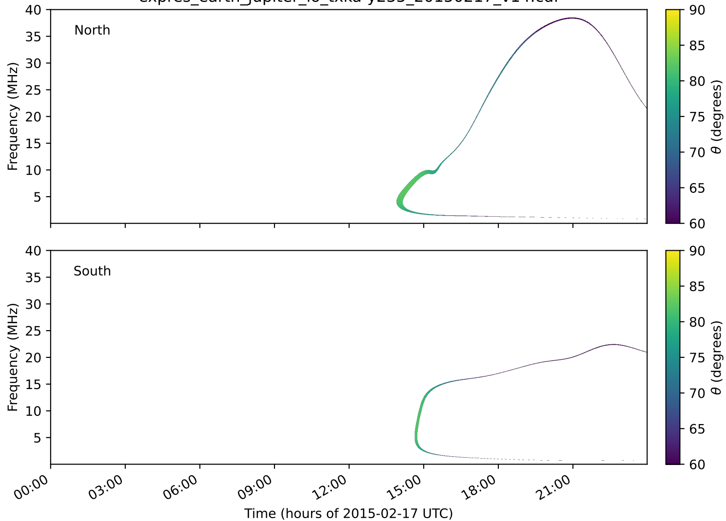
expres_earth_jupiter_io_txka-y235_20150217_v14.cdf
