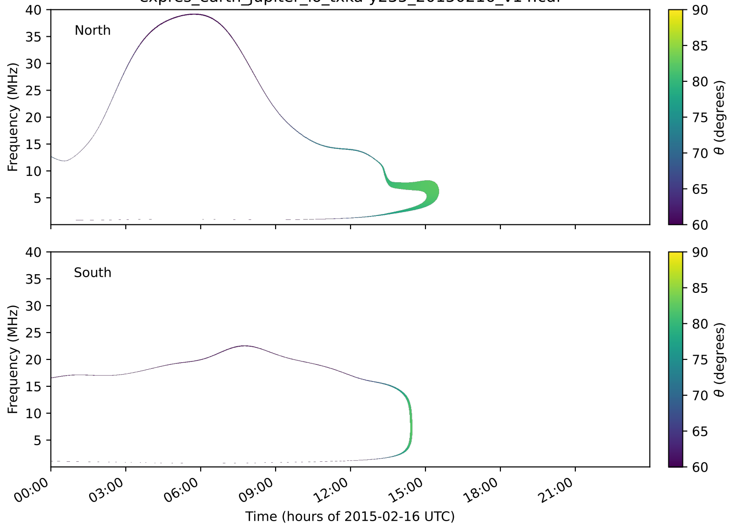
expres_earth_jupiter_io_txka-y235_20150216_v14.cdf
