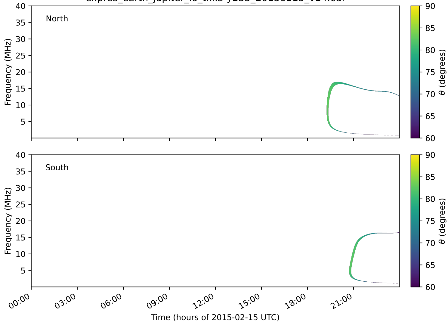
expres_earth_jupiter_io_txka-y235_20150215_v14.cdf
