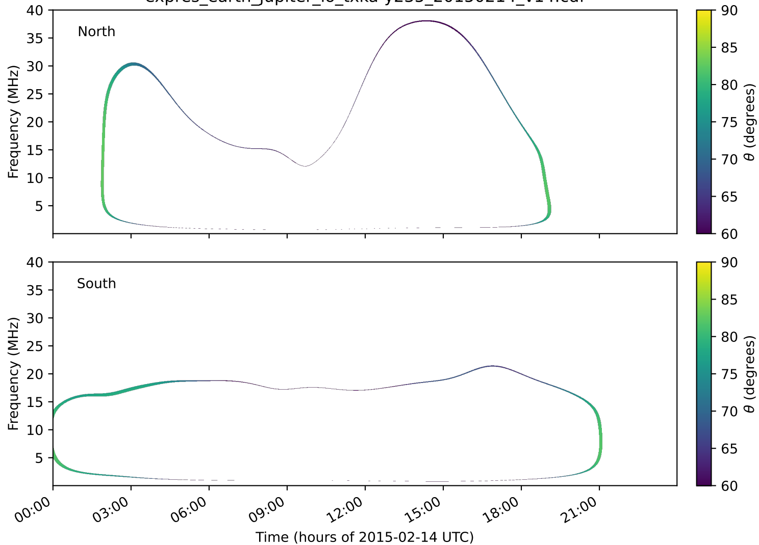
expres_earth_jupiter_io_txka-y235_20150214_v14.cdf
