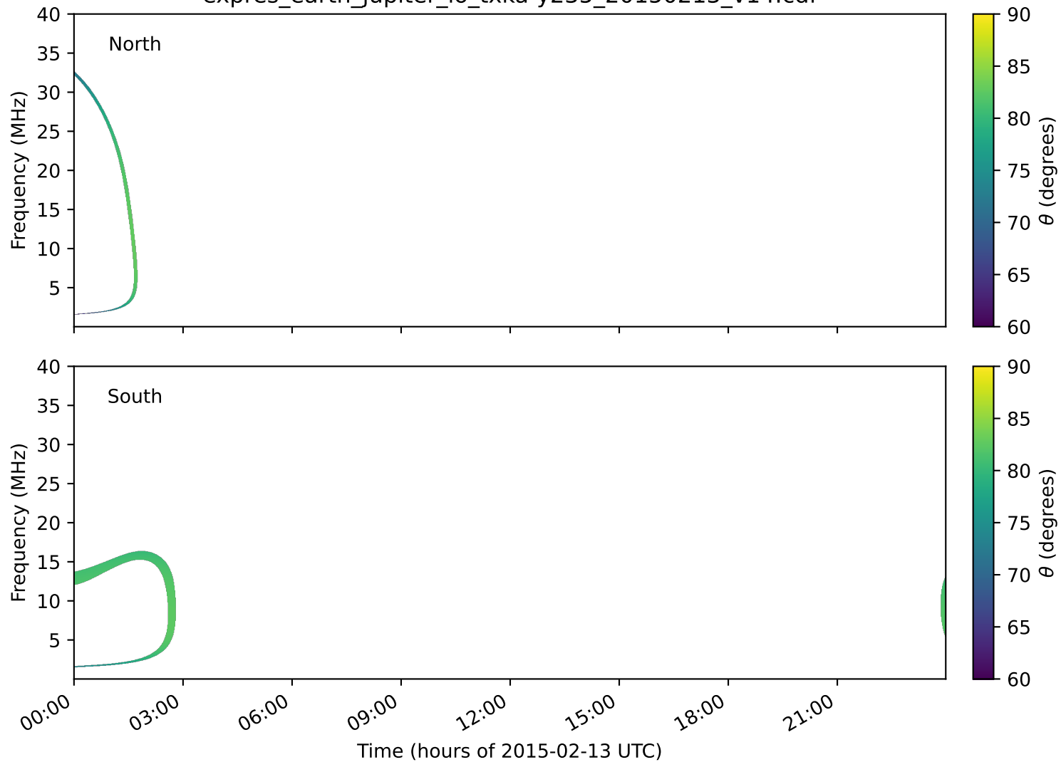
expres_earth_jupiter_io_txka-y235_20150213_v14.cdf
