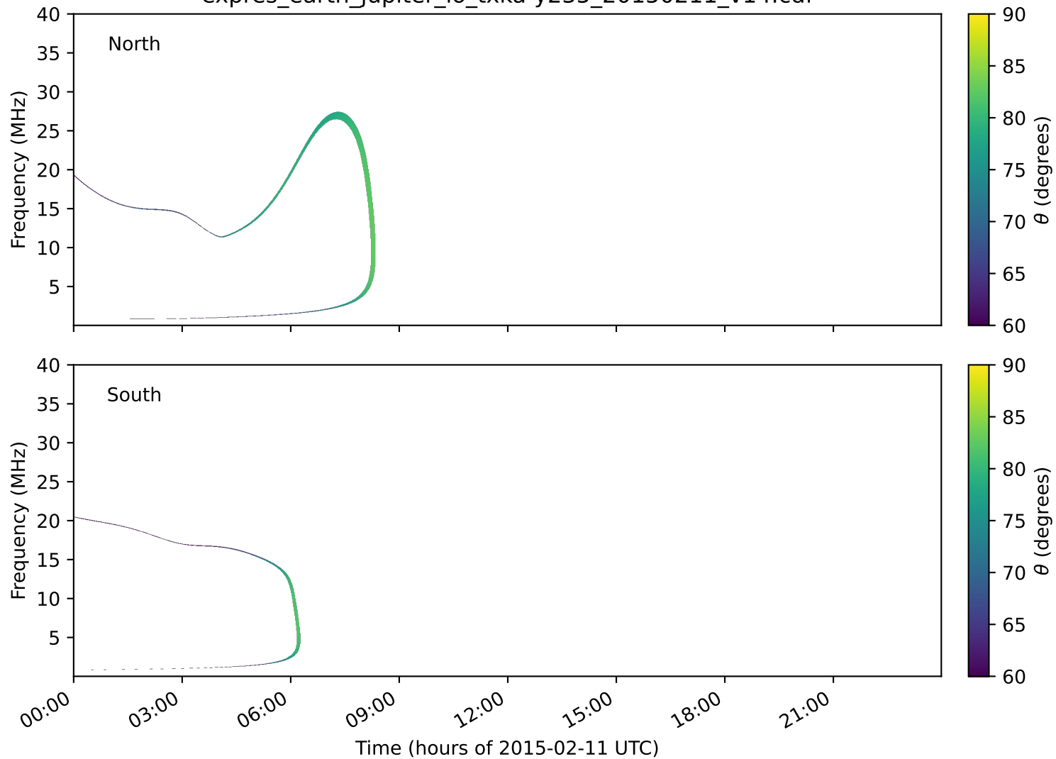
expres_earth_jupiter_io_txka-y235_20150211_v14.cdf
