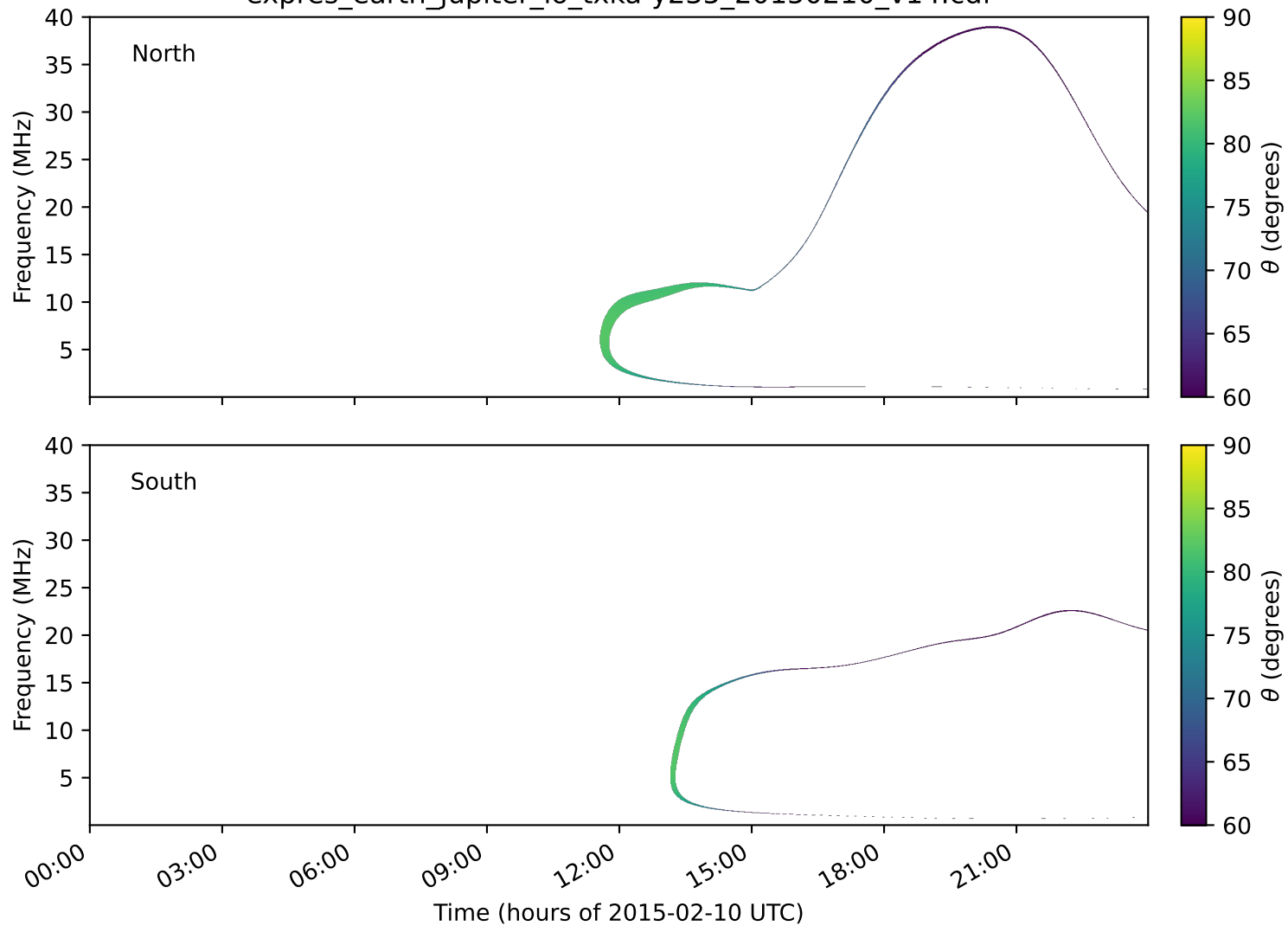
expres_earth_jupiter_io_txka-y235_20150210_v14.cdf
