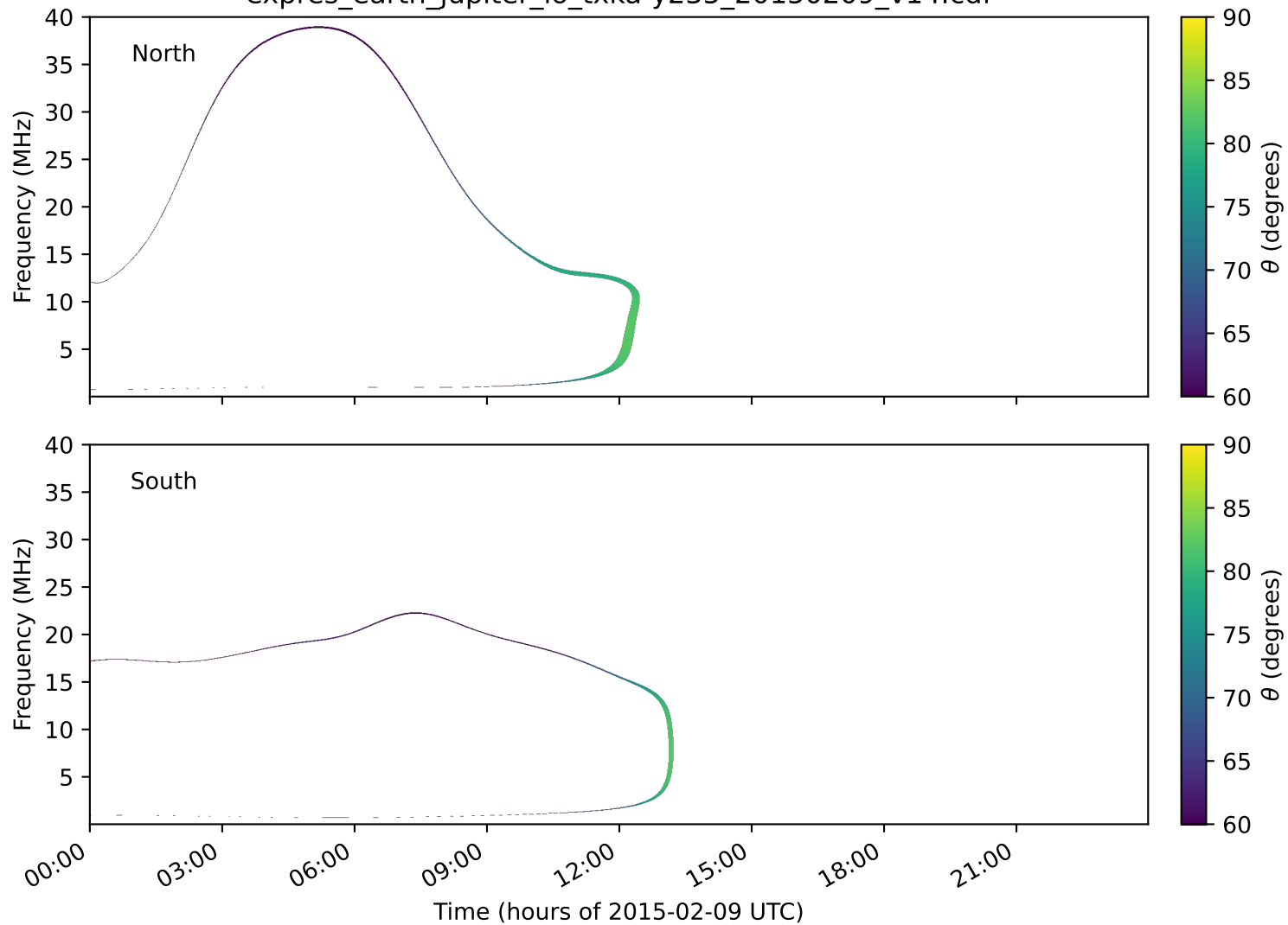
expres_earth_jupiter_io_txka-y235_20150209_v14.cdf
