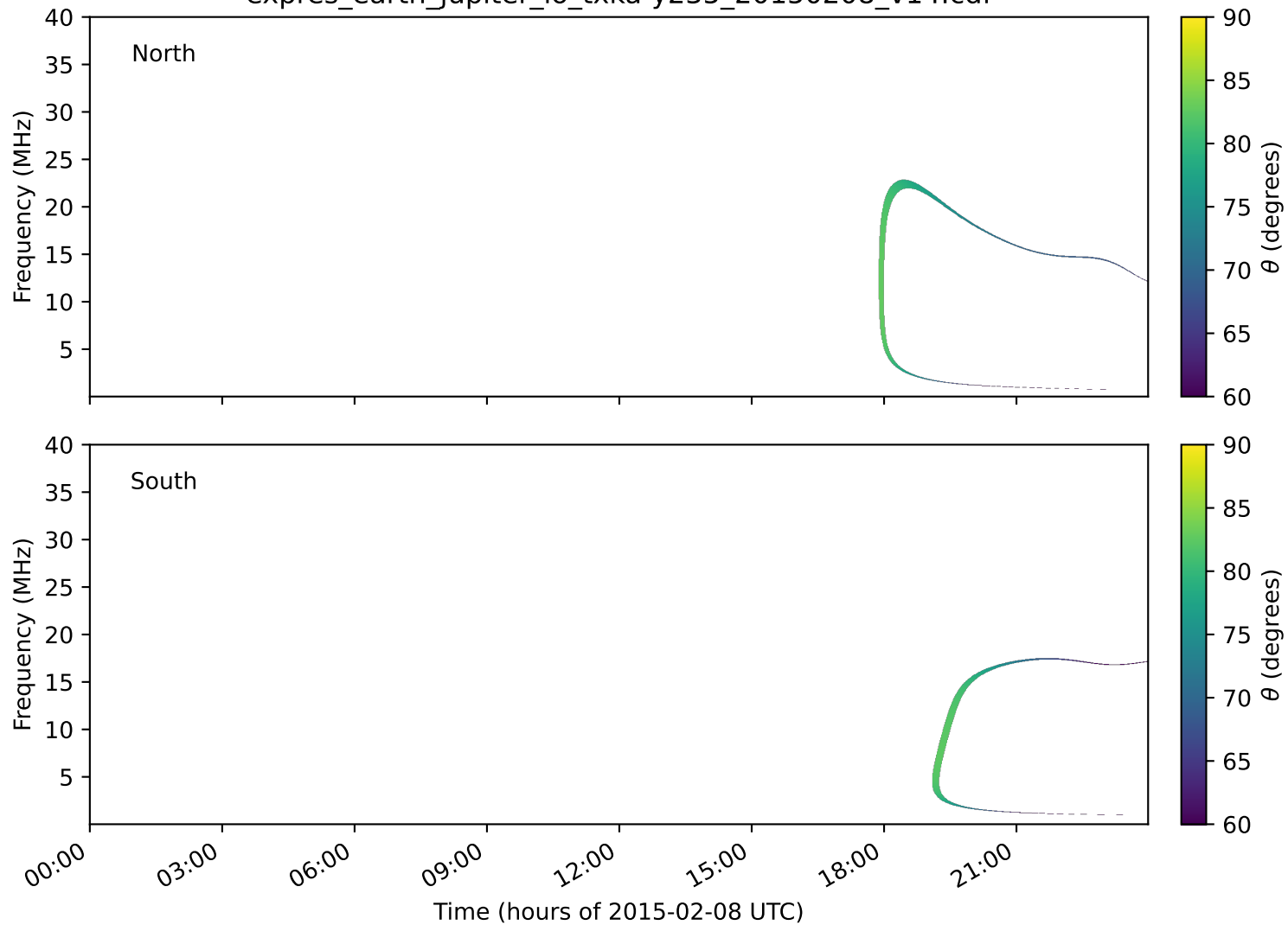
expres_earth_jupiter_io_txka-y235_20150208_v14.cdf
