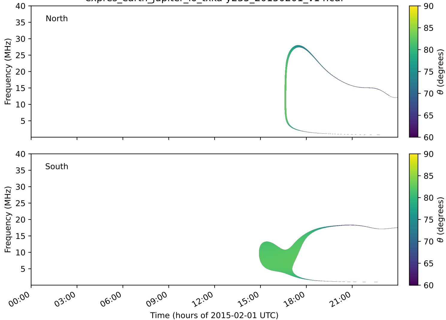
expres_earth_jupiter_io_txka-y235_20150201_v14.cdf
