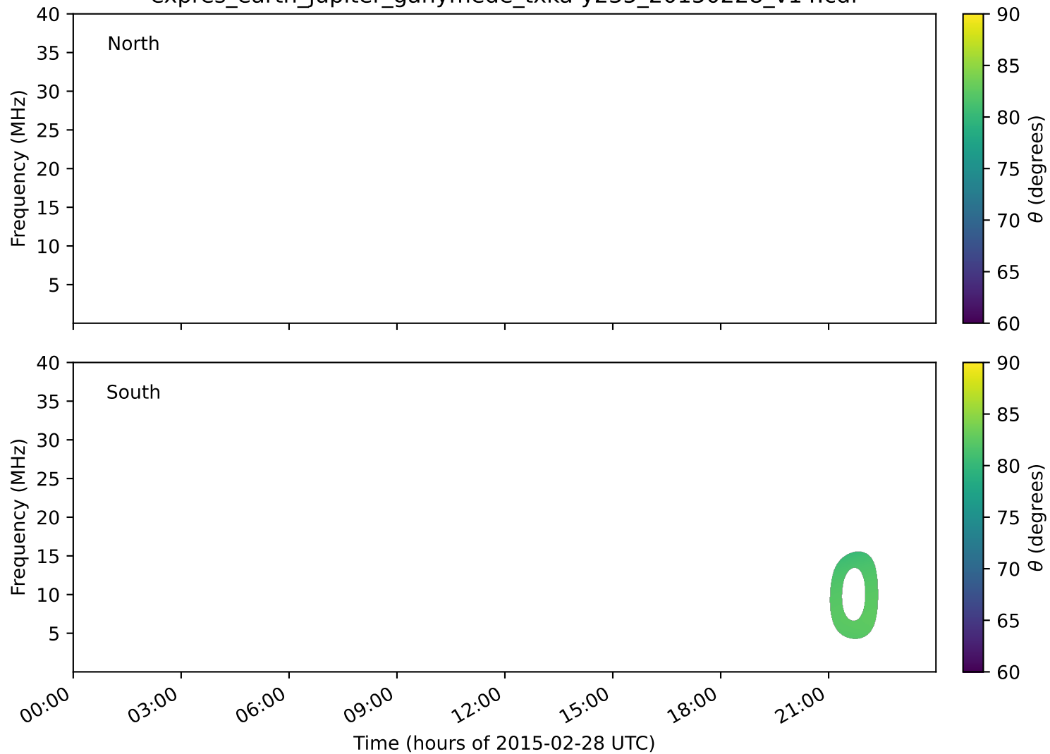
expres_earth_jupiter_ganymede_txka-y235_20150228_v14.cdf
