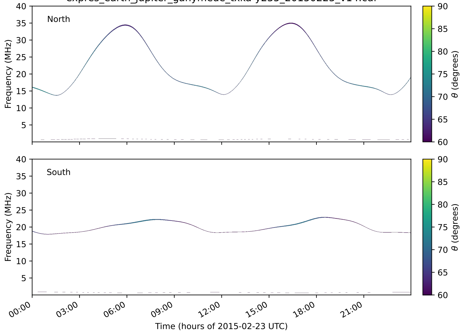
expres_earth_jupiter_ganymede_txka-y235_20150223_v14.cdf
