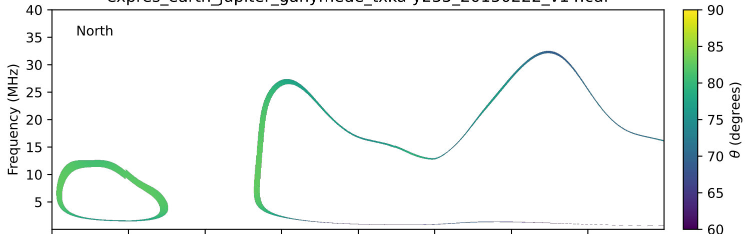
expres_earth_jupiter_ganymede_txka-y235_20150222_v14.cdf
