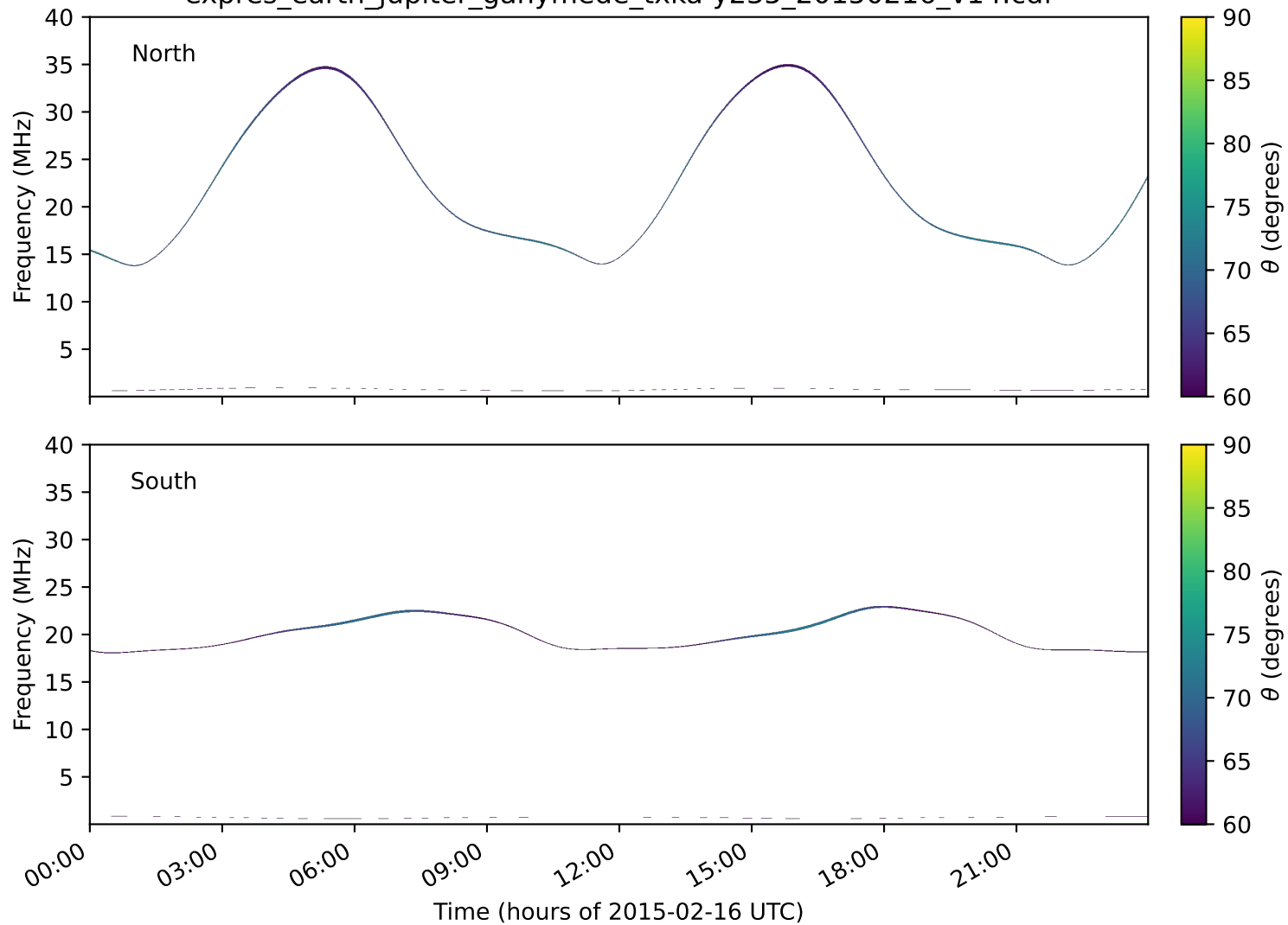
expres_earth_jupiter_ganymede_txka-y235_20150216_v14.cdf
