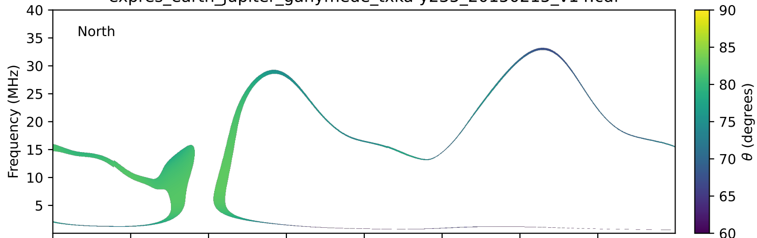
expres_earth_jupiter_ganymede_txka-y235_20150215_v14.cdf
