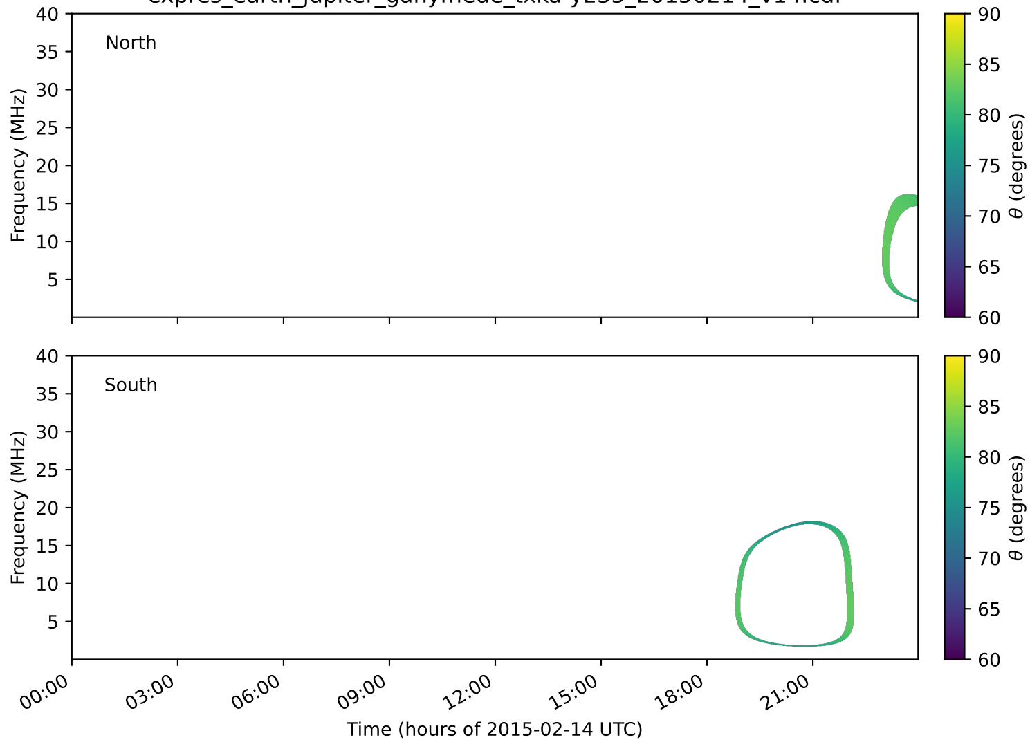
expres_earth_jupiter_ganymede_txka-y235_20150214_v14.cdf
