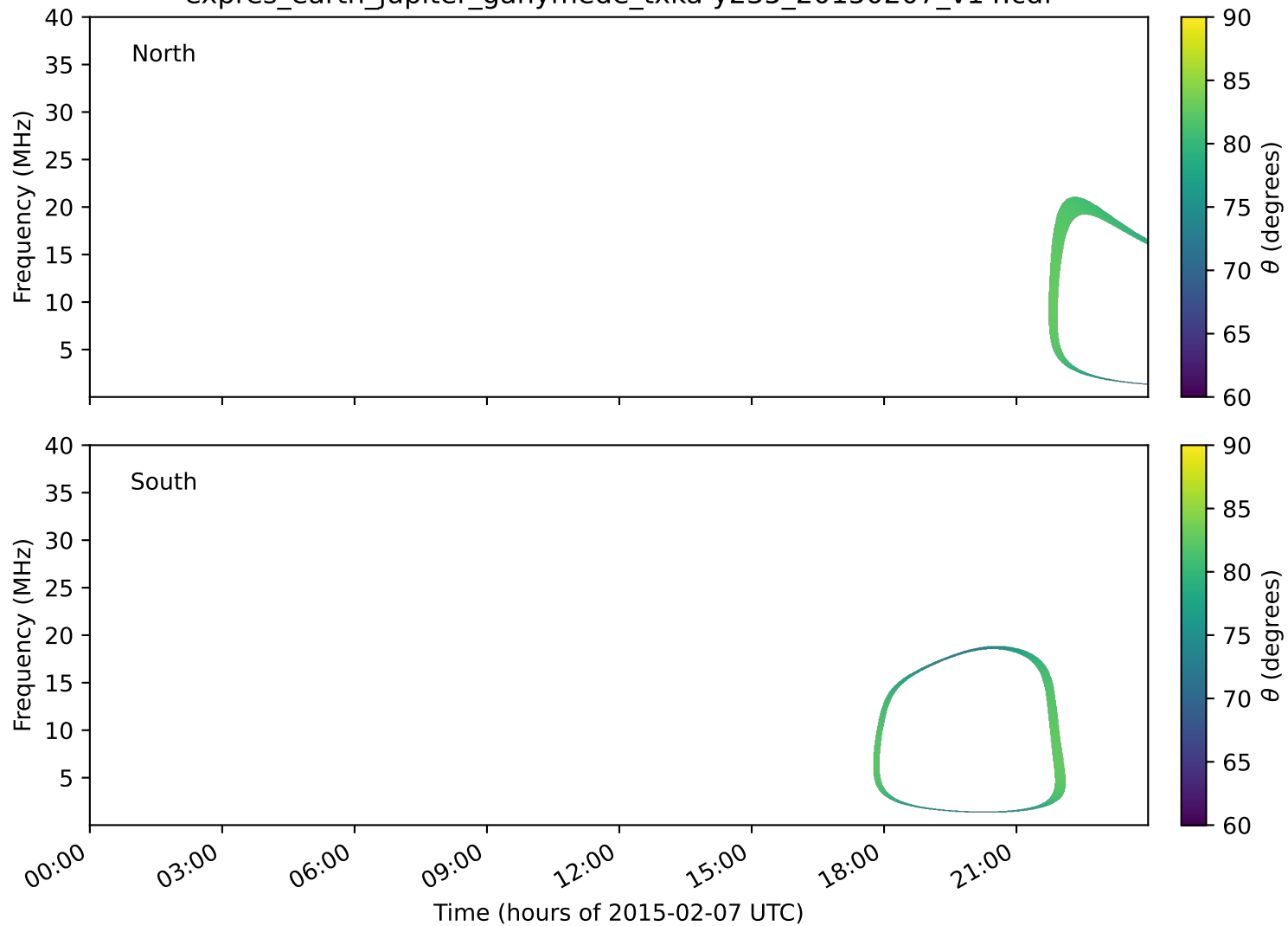
expres_earth_jupiter_ganymede_txka-y235_20150207_v14.cdf
