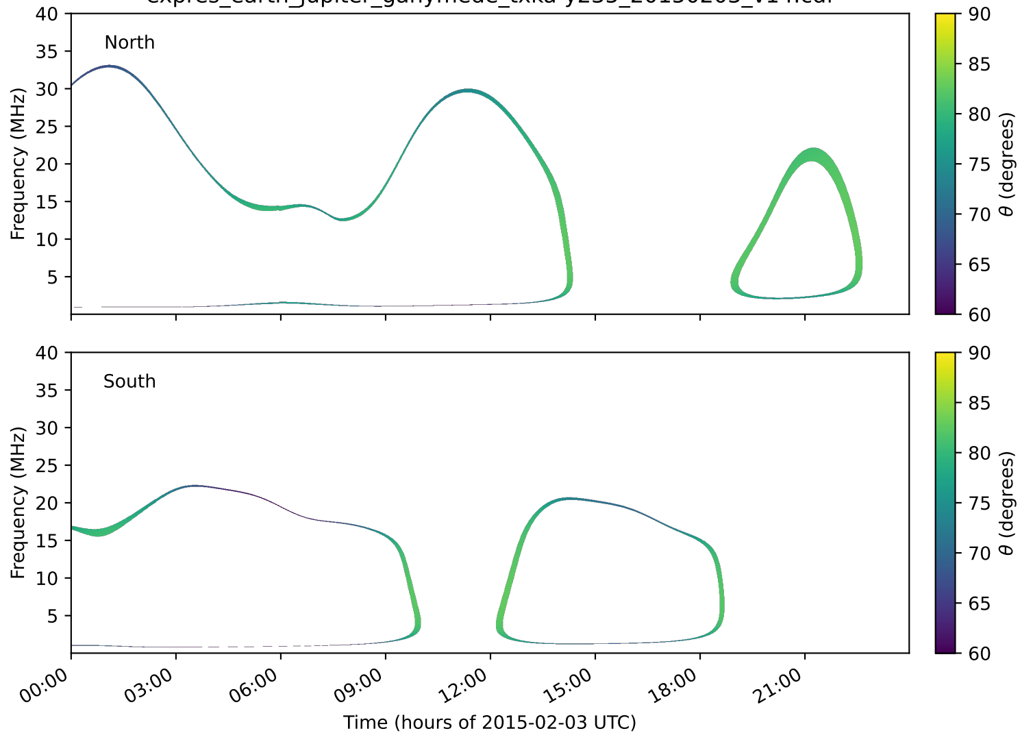
expres_earth_jupiter_ganymede_txka-y235_20150203_v14.cdf
