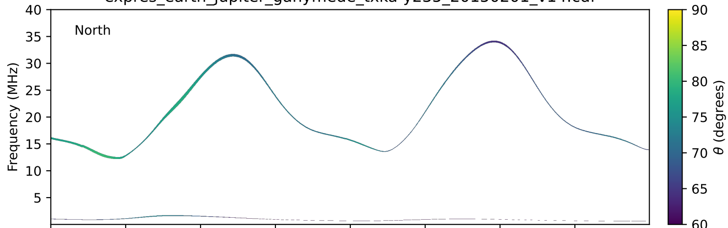
expres_earth_jupiter_ganymede_txka-y235_20150201_v14.cdf
