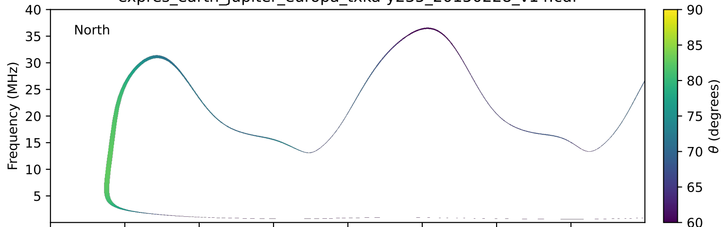
expres_earth_jupiter_europa_txka-y235_20150228_v14.cdf
