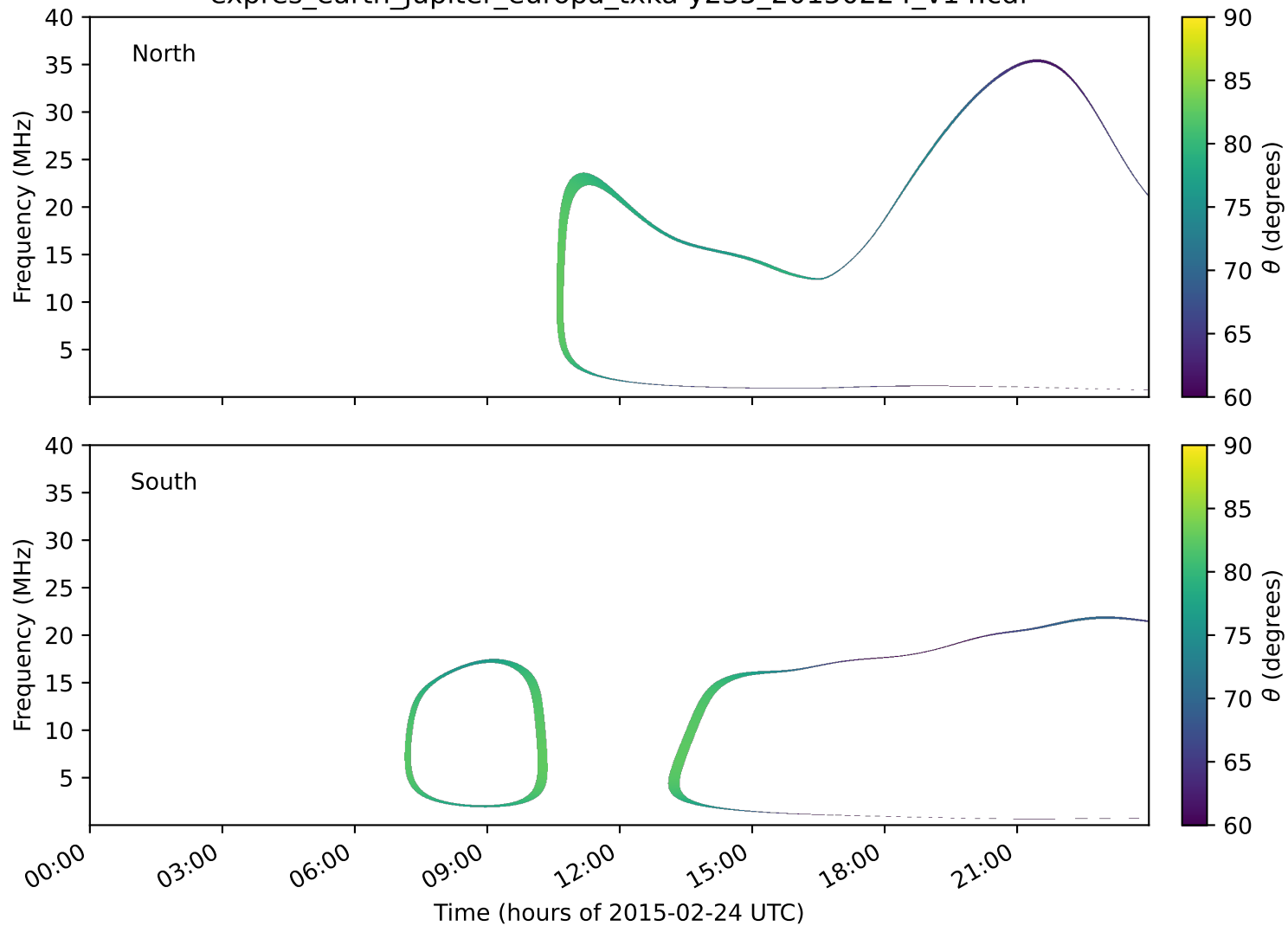
expres_earth_jupiter_europa_txka-y235_20150224_v14.cdf
