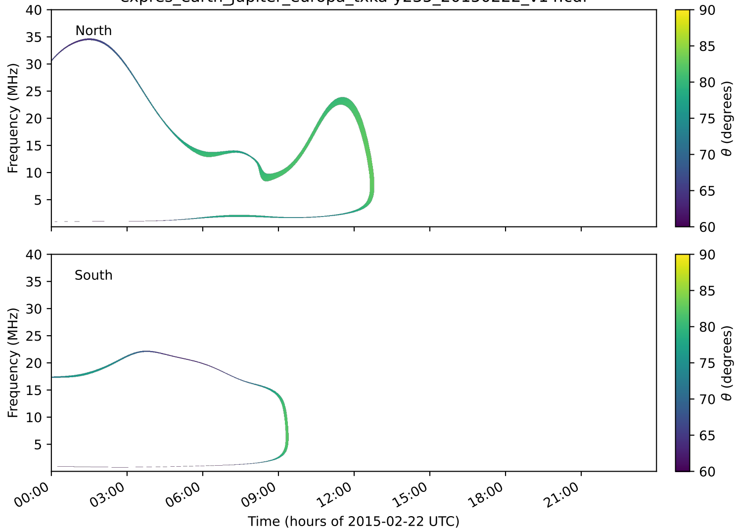
expres_earth_jupiter_europa_txka-y235_20150222_v14.cdf
