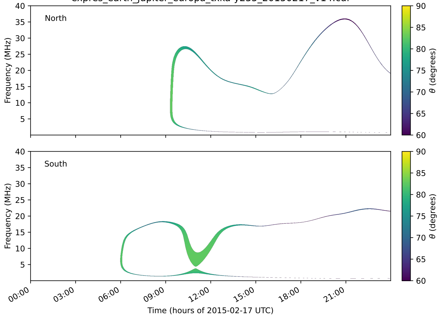
expres_earth_jupiter_europa_txka-y235_20150217_v14.cdf
