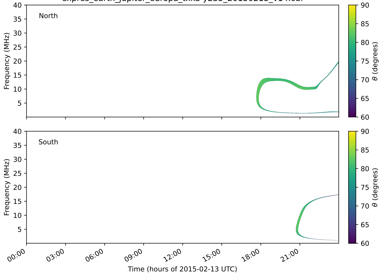
expres_earth_jupiter_europa_txka-y235_20150213_v14.cdf
