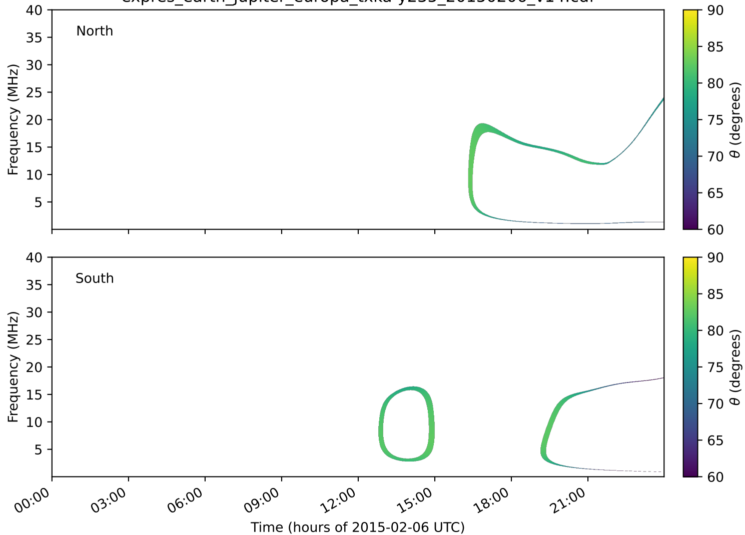
expres_earth_jupiter_europa_txka-y235_20150206_v14.cdf
