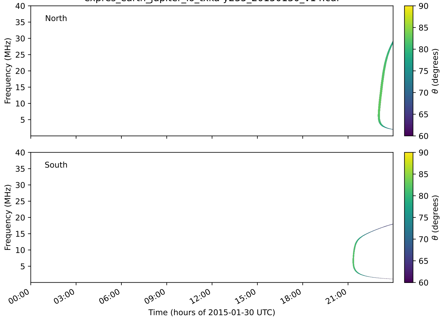
expres_earth_jupiter_io_txka-y235_20150130_v14.cdf
