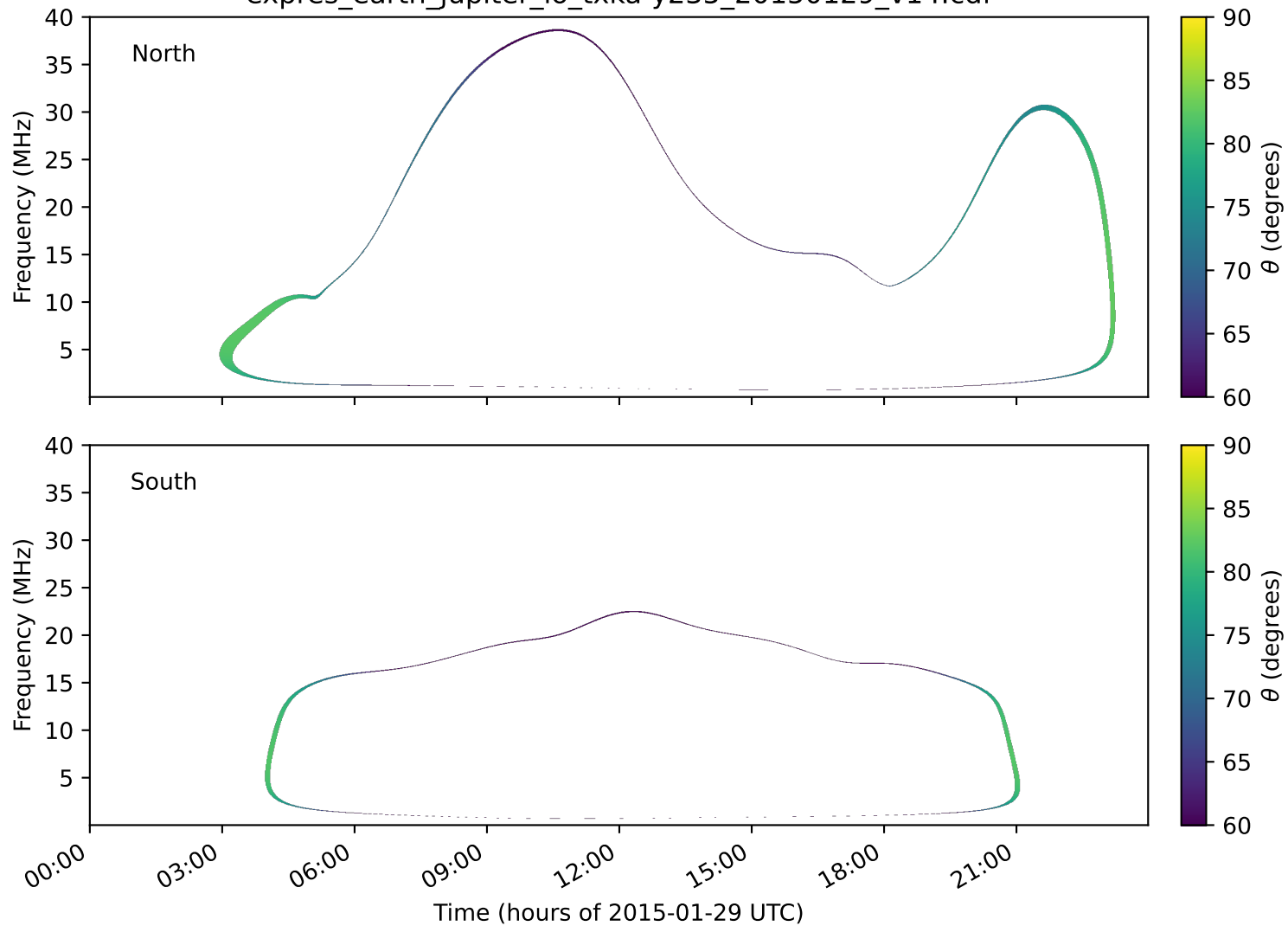
expres_earth_jupiter_io_txka-y235_20150129_v14.cdf
