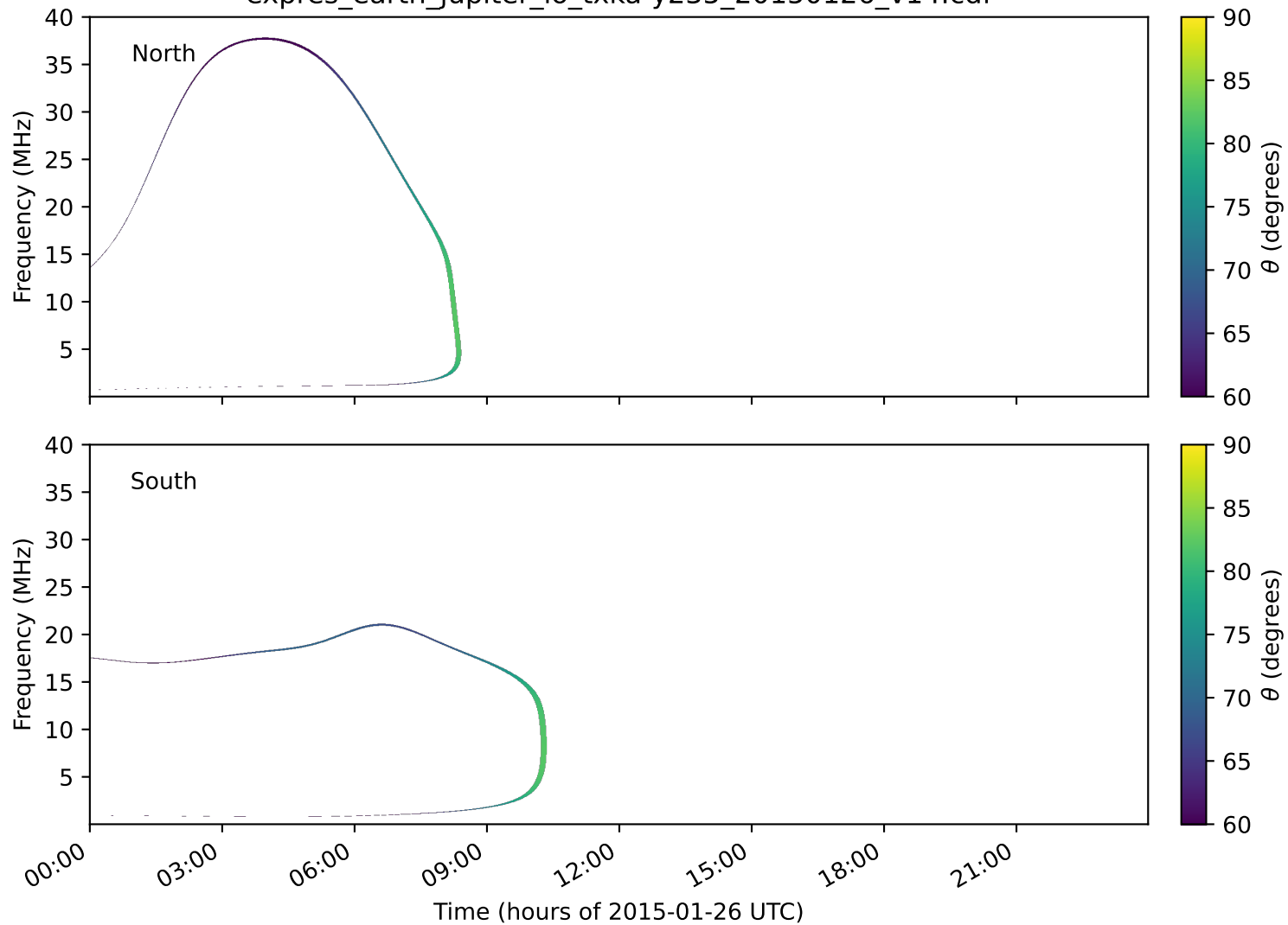
expres_earth_jupiter_io_txka-y235_20150126_v14.cdf
