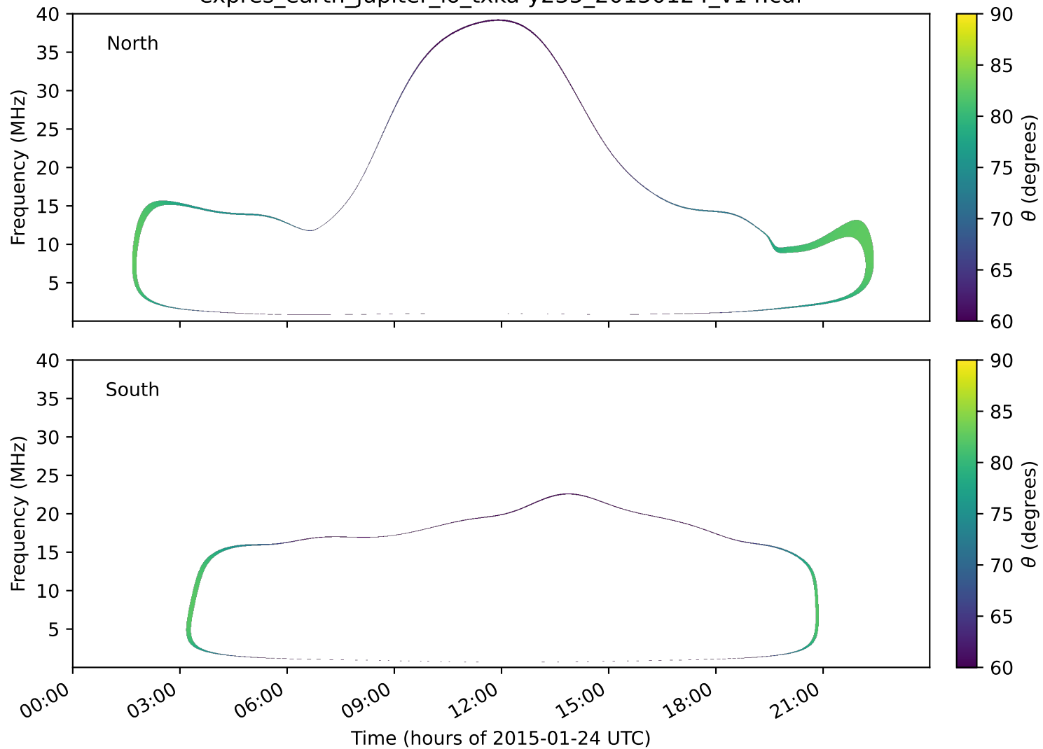
expres_earth_jupiter_io_txka-y235_20150124_v14.cdf
