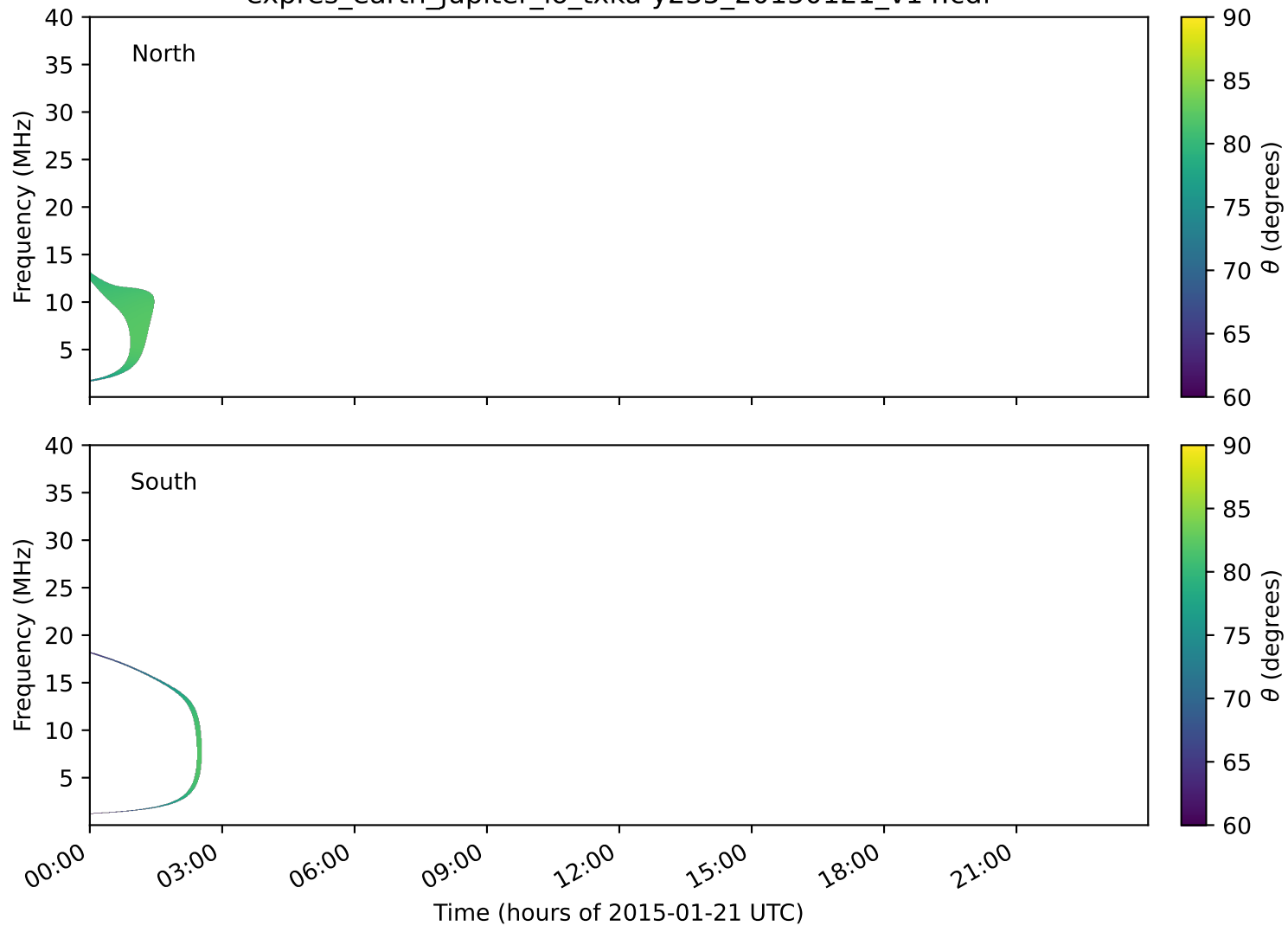
expres_earth_jupiter_io_txka-y235_20150121_v14.cdf
