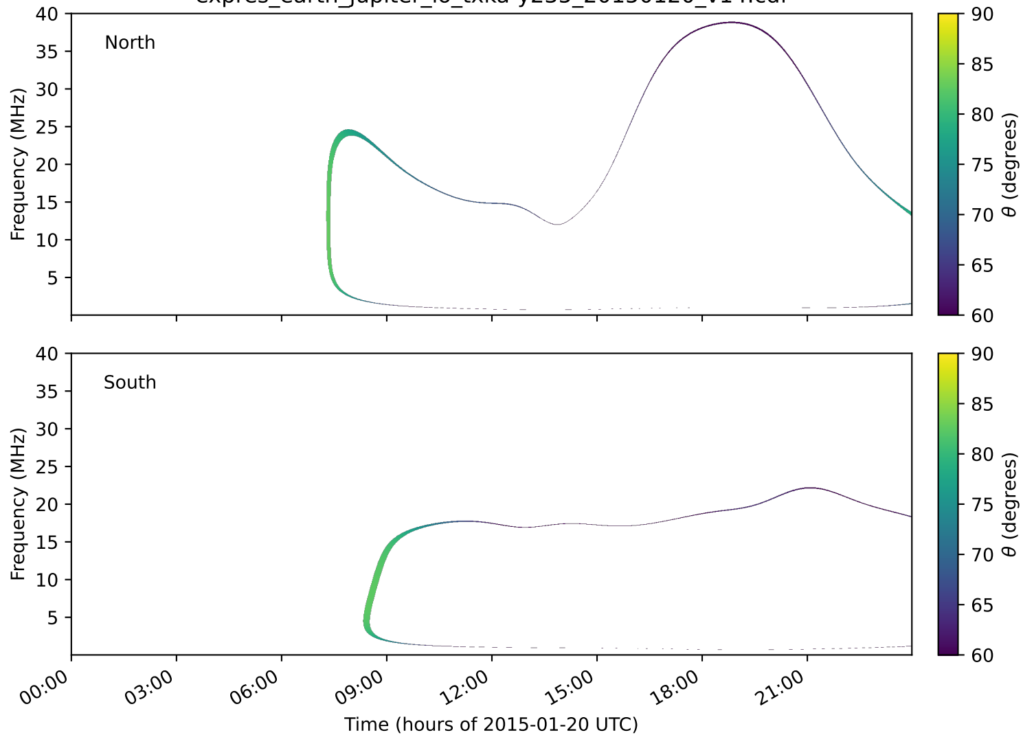
expres_earth_jupiter_io_txka-y235_20150120_v14.cdf
