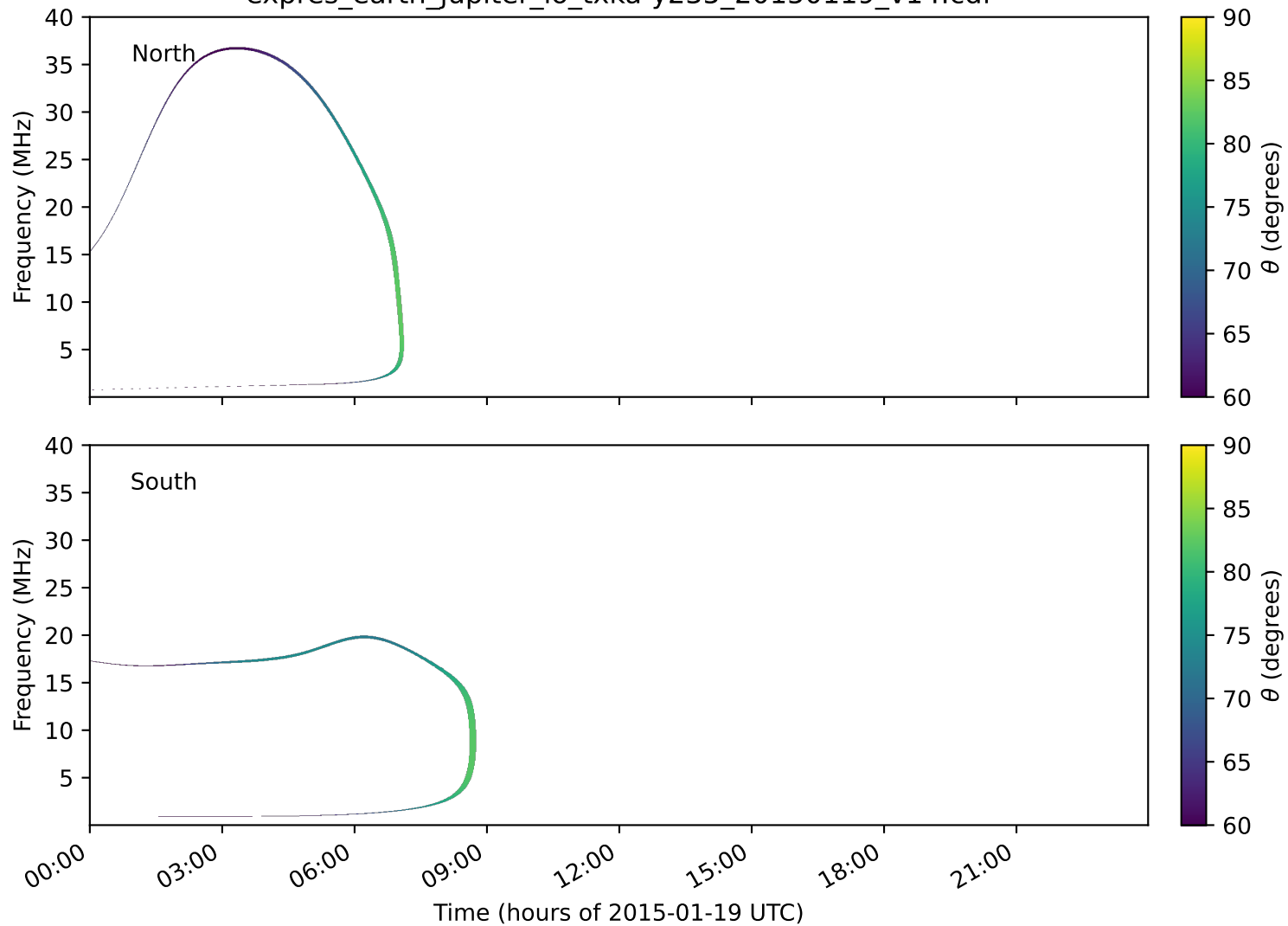
expres_earth_jupiter_io_txka-y235_20150119_v14.cdf
