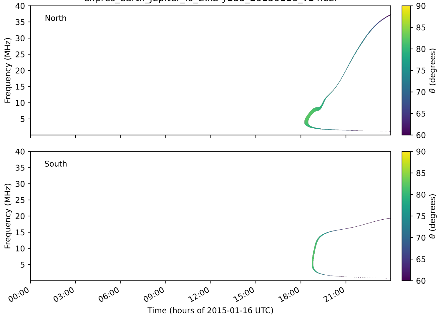
expres_earth_jupiter_io_txka-y235_20150116_v14.cdf
