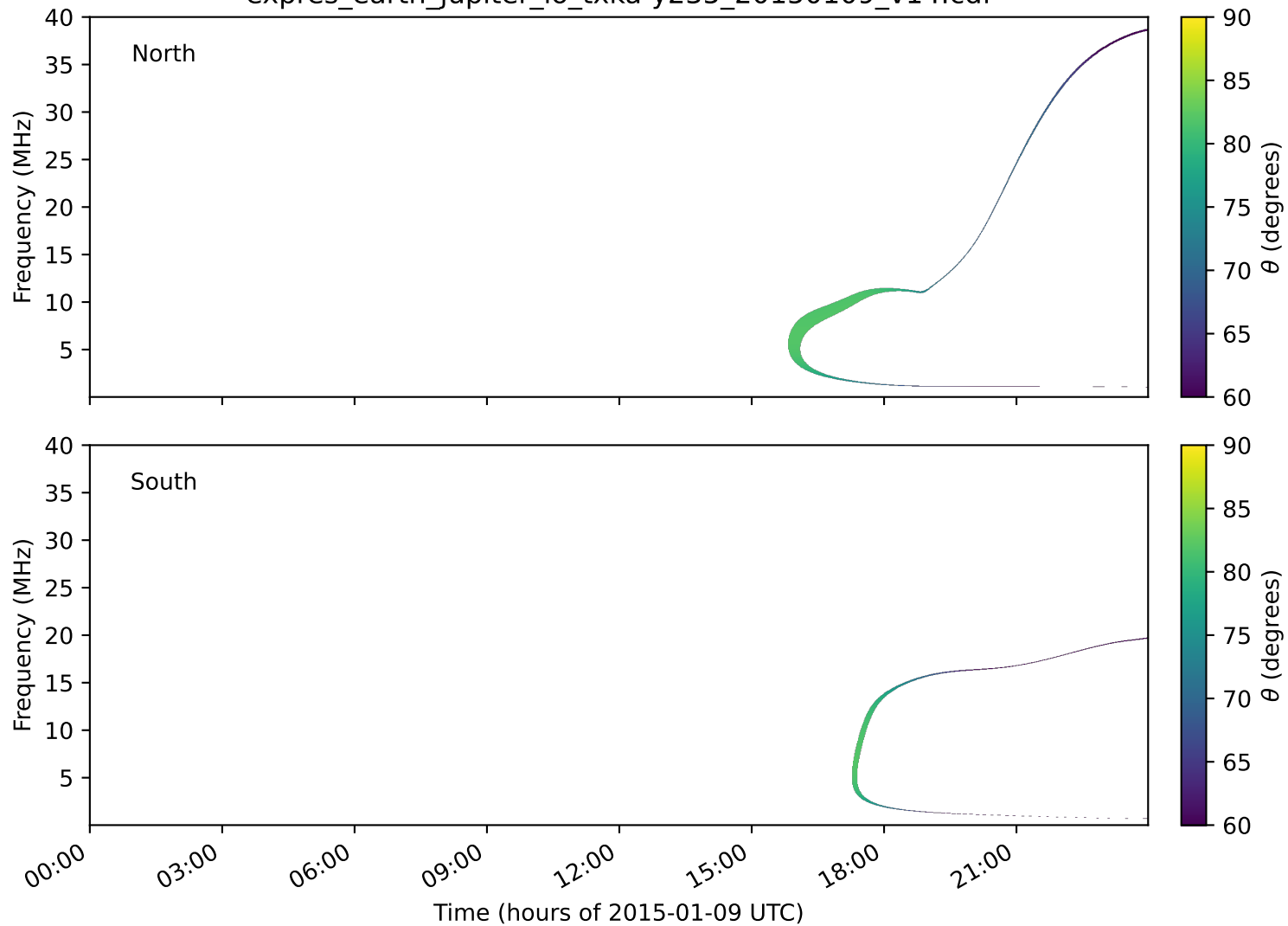
expres_earth_jupiter_io_txka-y235_20150109_v14.cdf
