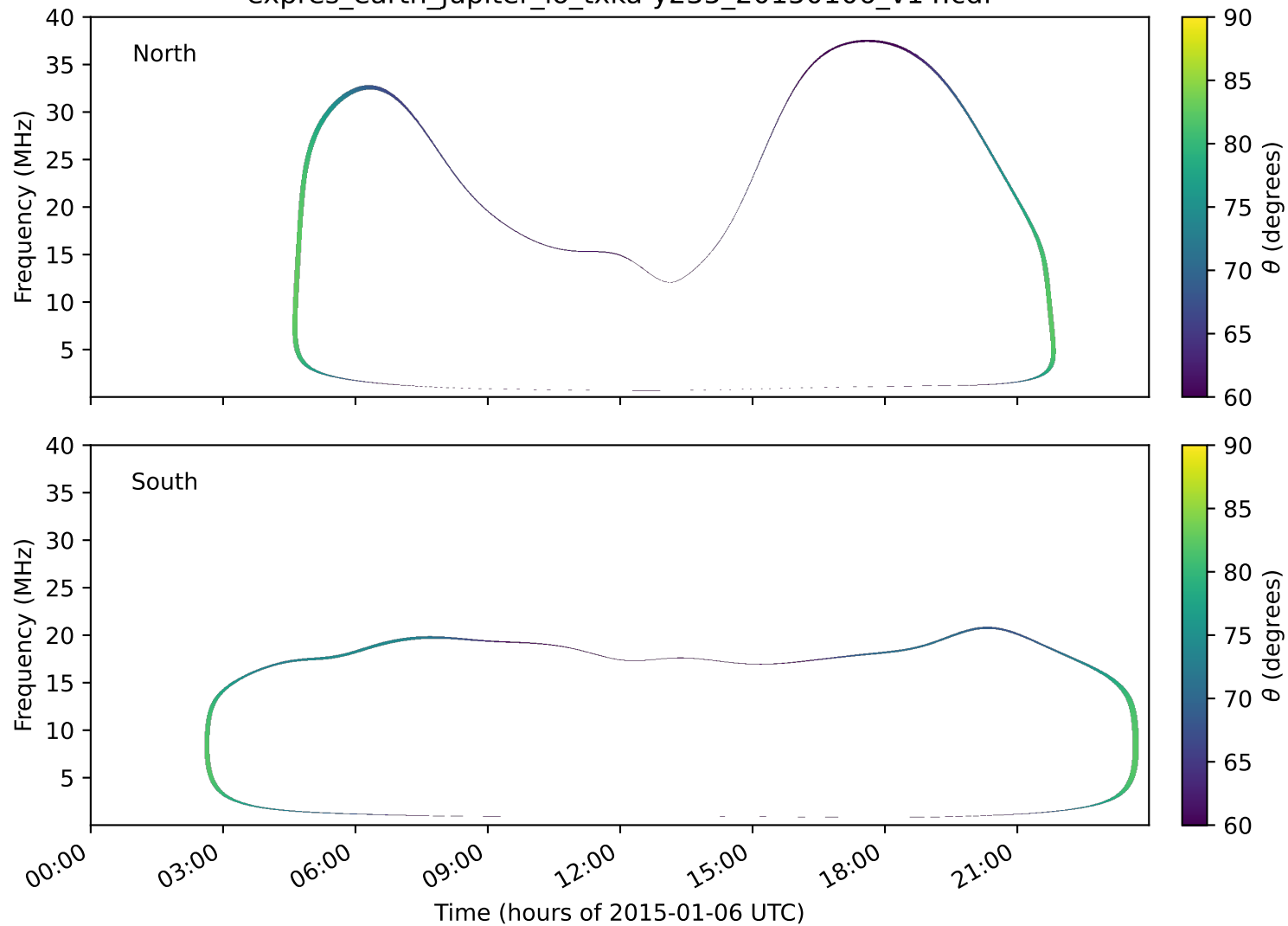
expres_earth_jupiter_io_txka-y235_20150106_v14.cdf
