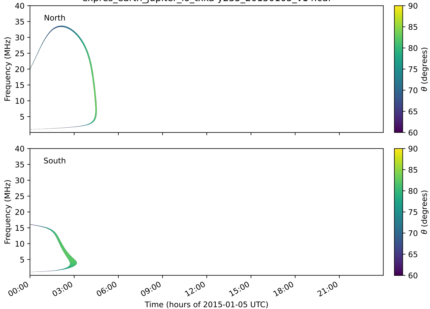
expres_earth_jupiter_io_txka-y235_20150105_v14.cdf
