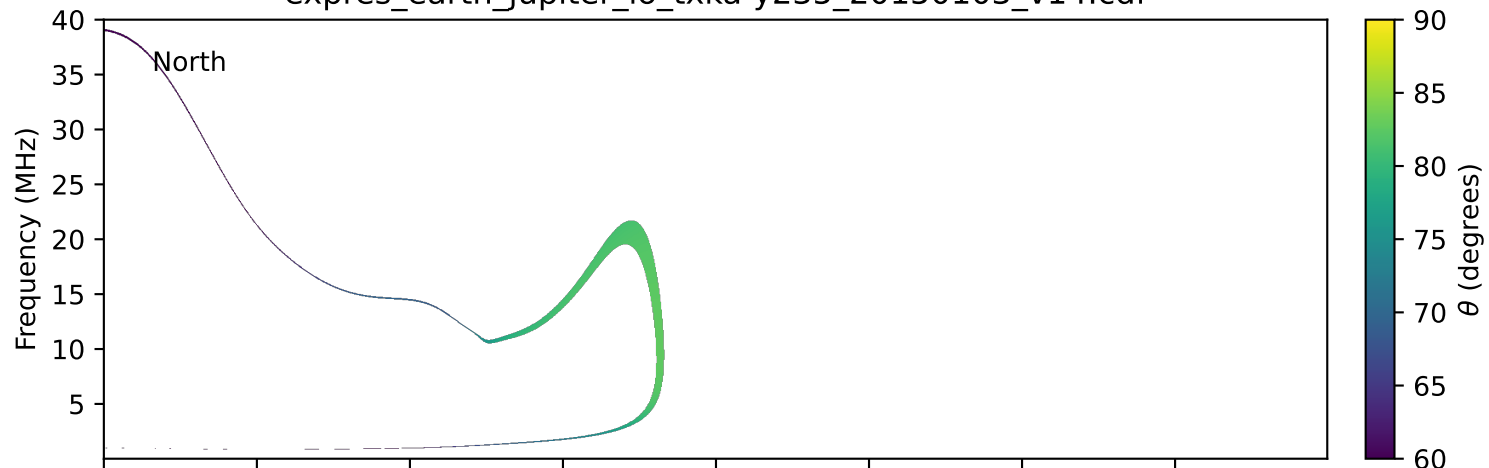
expres_earth_jupiter_io_txka-y235_20150103_v14.cdf
