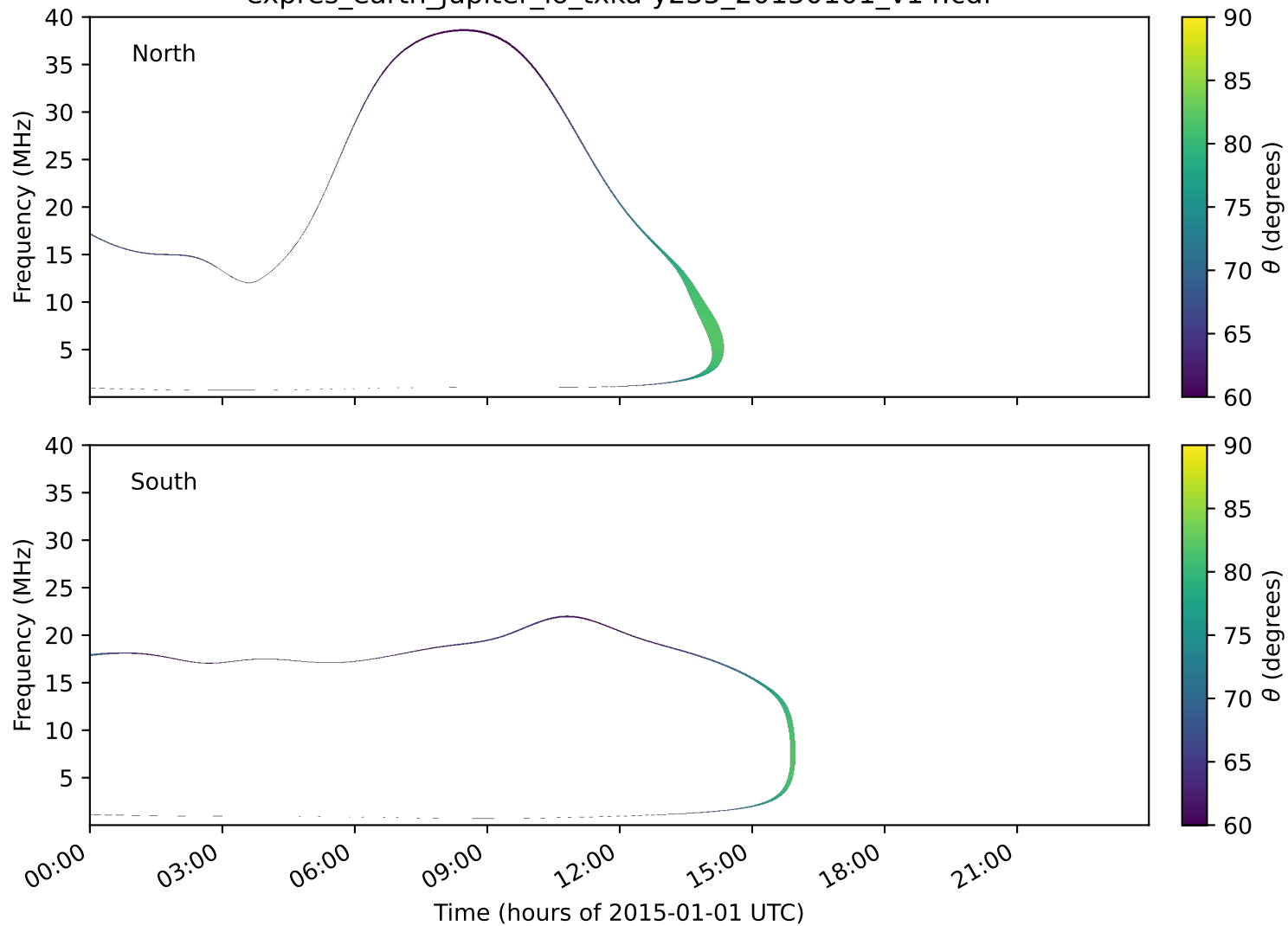
expres_earth_jupiter_io_txka-y235_20150101_v14.cdf
