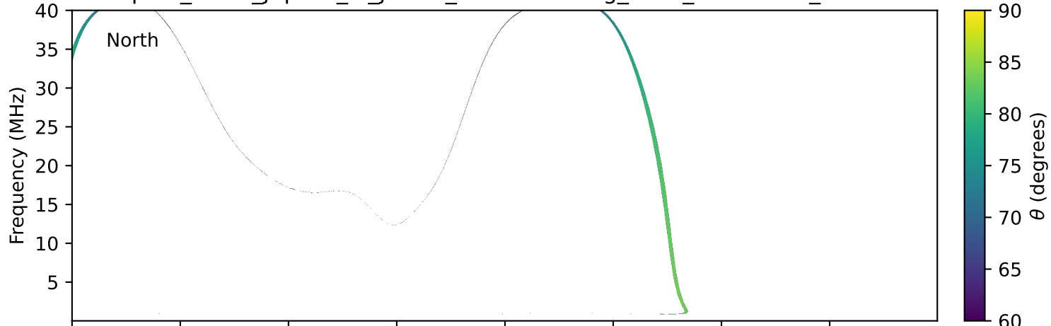
expres_earth_jupiter_io_jrm33_lossc-wid1deg_3kev_20150131_v11.cdf
