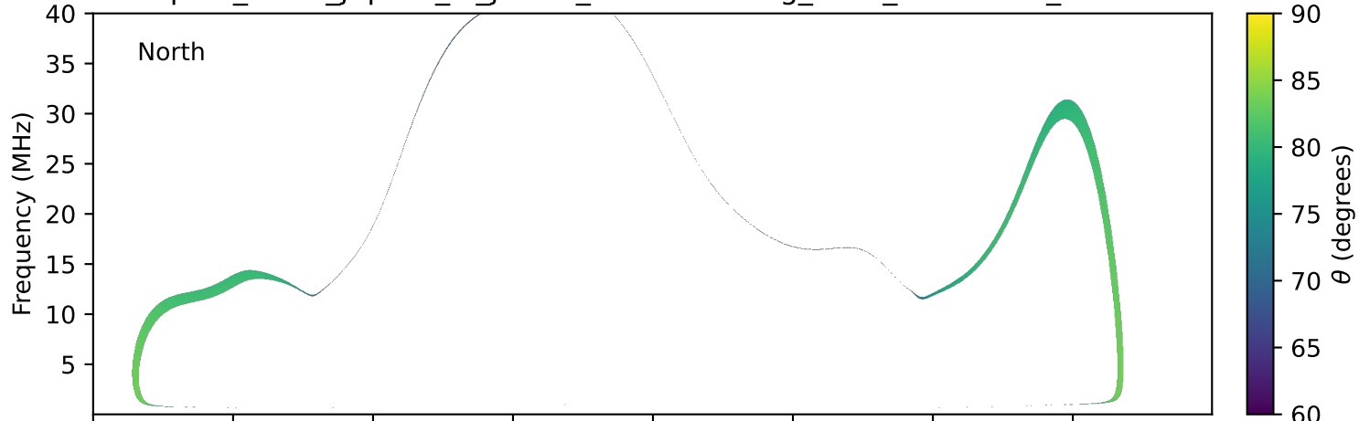
expres_earth_jupiter_io_jrm33_lossc-wid1deg_3kev_20150122_v11.cdf
