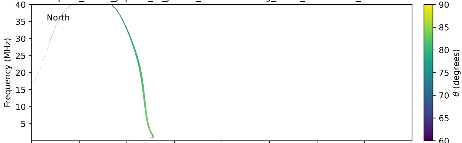
expres_earth_jupiter_io_jrm33_lossc-wid1deg_3kev_20150119_v11.cdf
