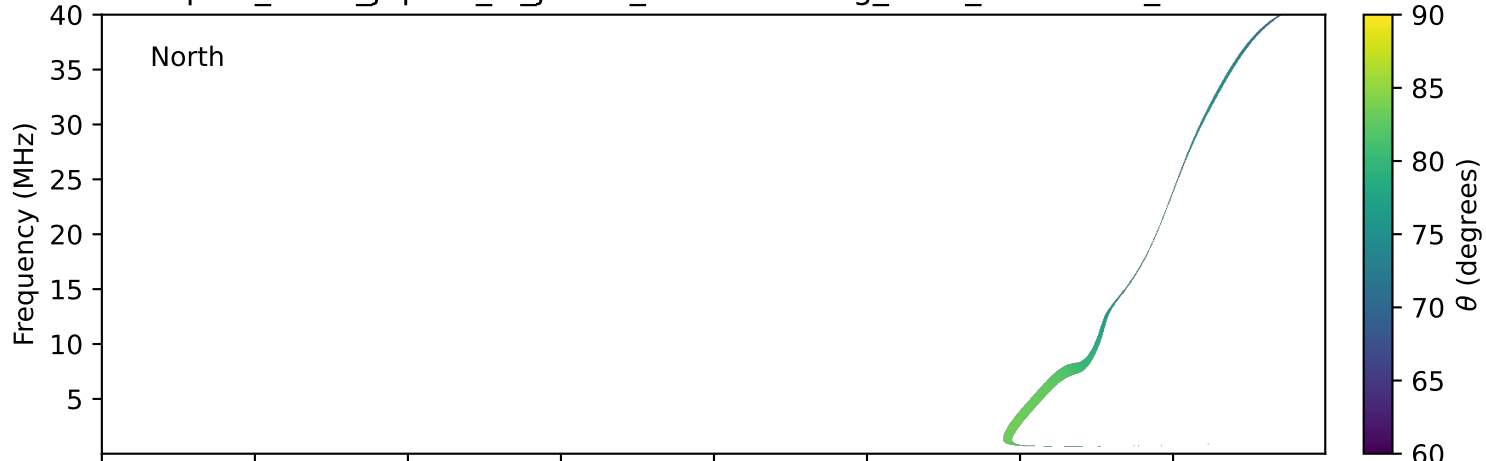
expres_earth_jupiter_io_jrm33_lossc-wid1deg_3kev_20150116_v11.cdf
