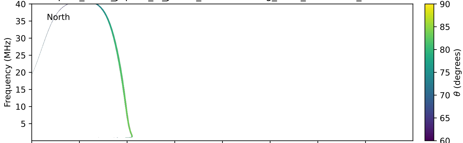
expres_earth_jupiter_io_jrm33_lossc-wid1deg_3kev_20150112_v11.cdf
