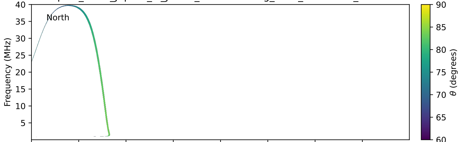
expres_earth_jupiter_io_jrm33_lossc-wid1deg_3kev_20150105_v11.cdf
